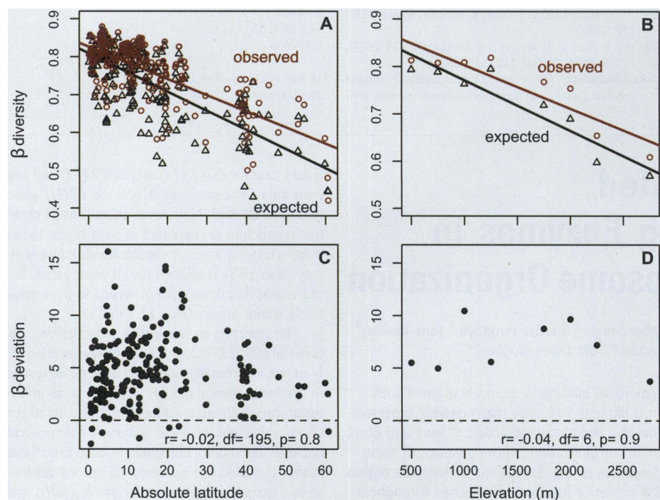
Fig. 3. Patterns in observed (red) and expected (black) \beta diversity of woody plants along a latitudinal (A) and an elevational (B) gradient and patterns in the \beta deviation, a standard effect size of \beta -diversity deviations from a null model that corrects for \gamma dependence, with either latitude (C) or elevation (D).
